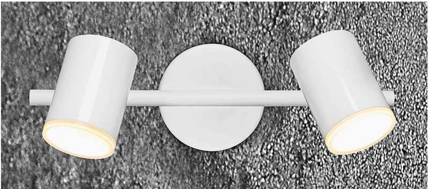
Art.nr W H COLOR 400719 30 16,5 White LED 2x5W 230V 3000K
