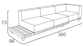
TC-18-TA TOUCH 3 SEATER CORNER RIGHT END W300 D96 H73 CBM: 2.00
