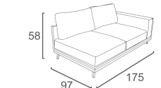
LAZ-05-TA LAZY 2 SEATER LEFT END W175 D97 H58 CBM: 0.87
